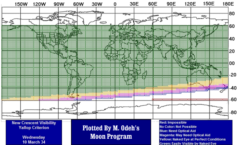
Figure 62: Nisan Visibility Plot for 3/10 AD 34
